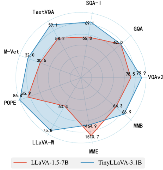
Figure 1.5: Benchmark comparison from TinyLLaVA Figure 1, where a 3.1B small-scale multi-modal model remains competitive with the 7B LLaVA-1.5 baseline across several benchmarks [23].
