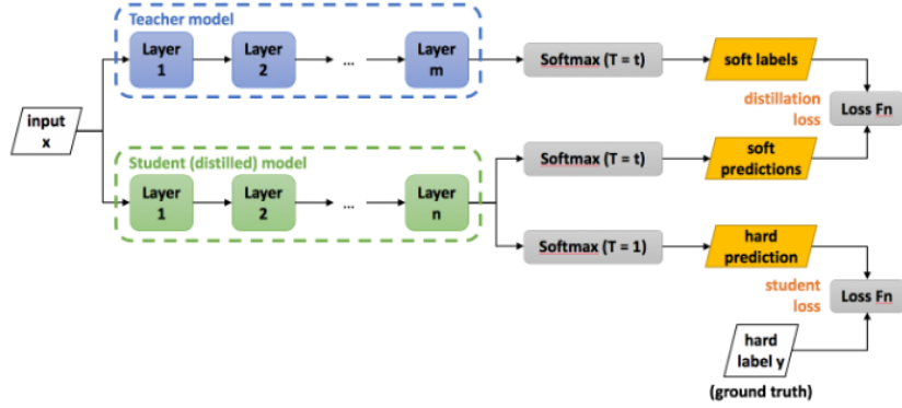
Figure 1.7: Knowledge distillation transfers information from a teacher model to a smaller student model [10, 11].
