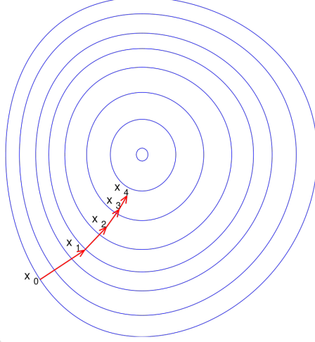
Figure 3.6: A directional view of gradient descent on a contour surface [51]. GRACE uses the same directional idea at the logit level: teachers whose KD update direction aligns better with the CE direction receive larger GRACE weights after warmup.
