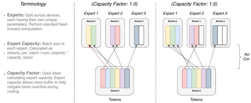
Figure 2.8: Illustration of sparse routing with expert capacity constraints, adapted from Switch Transformers [44]. Capacity factors control how many routed samples each expert can accept before overflow, which is directly analogous to the capacity-aware teacher routing used in GRACE.
