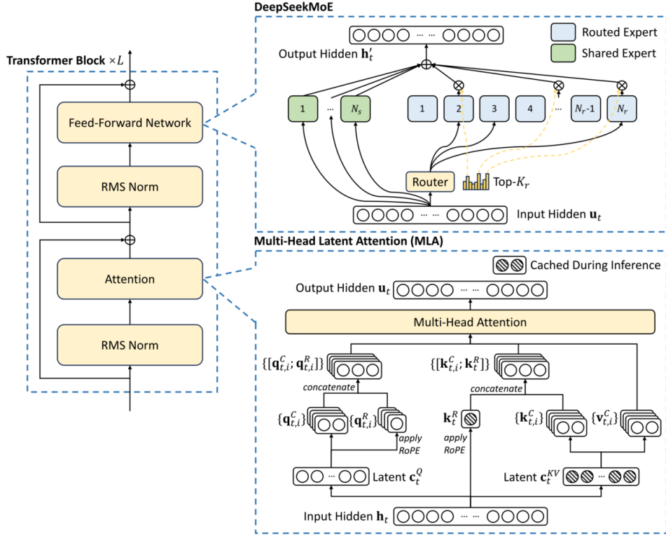
Figure 2.9: Example of sparse routing and expert specialization in a mixture-of-experts architecture [49, 50]. Although our setting is multi-teacher distillation rather than token-level MoE language modeling, the same principles of learned routing, sparse activation, and load balancing are directly relevant.
