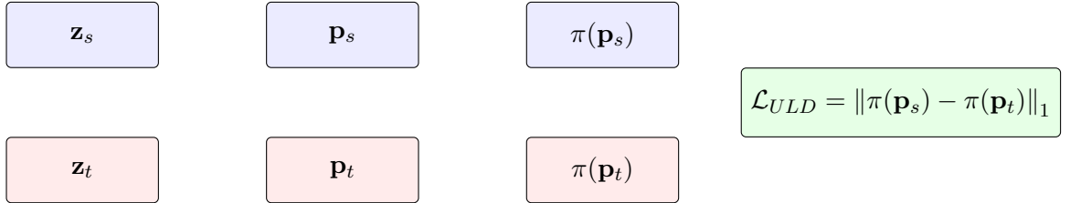
Figure 2.7: ULD compares ranked probability mass after temperature scaling, sorting, and zero-padding to a common vocabulary length [14].
