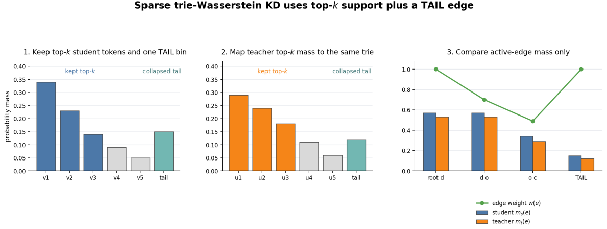
Figure 3.3: Sparse trie-Wasserstein support in the implementation.
