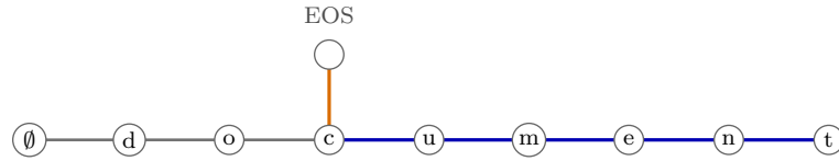
Figure 3.4: Trie split for document and doc .
