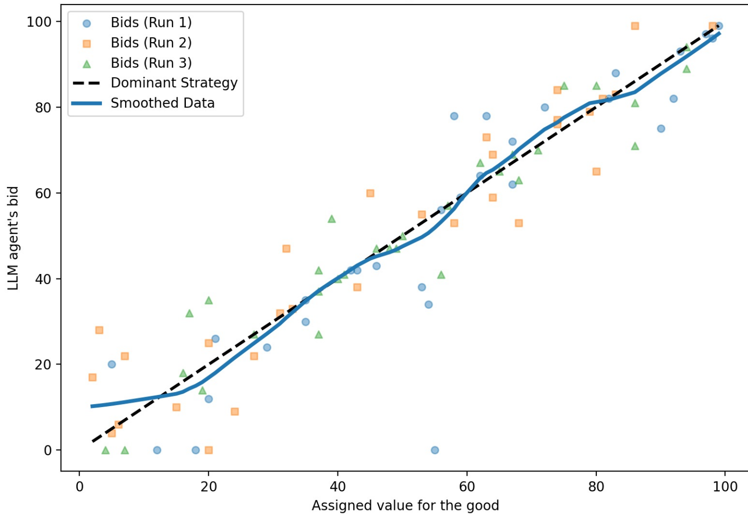
Second-Price: Assigned Value vs. Bid
