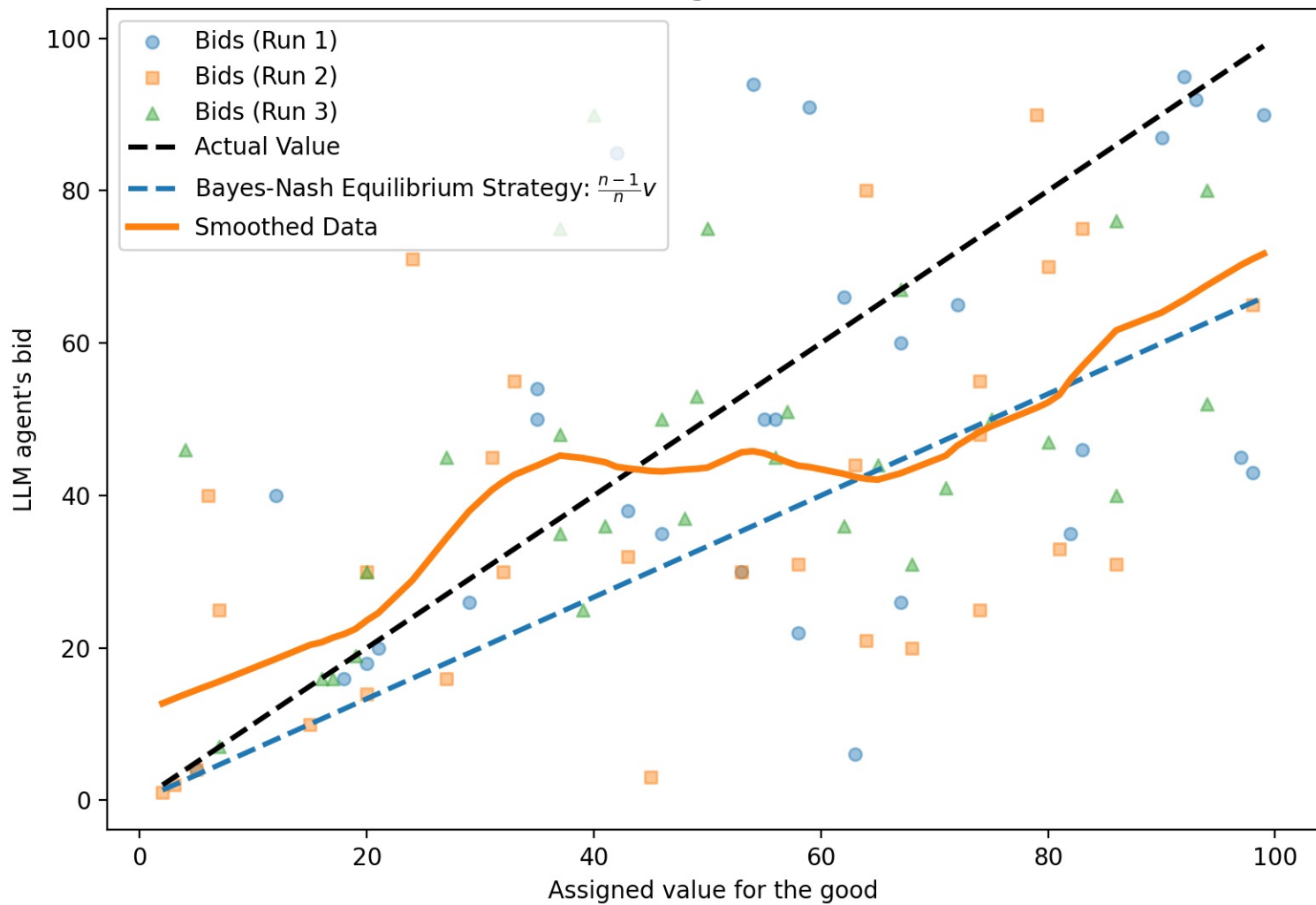
First-Price: Assigned Value vs. Bid
