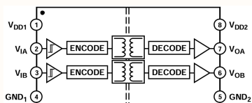
Figure 1. ADuM1200 Functional Block Diagram
