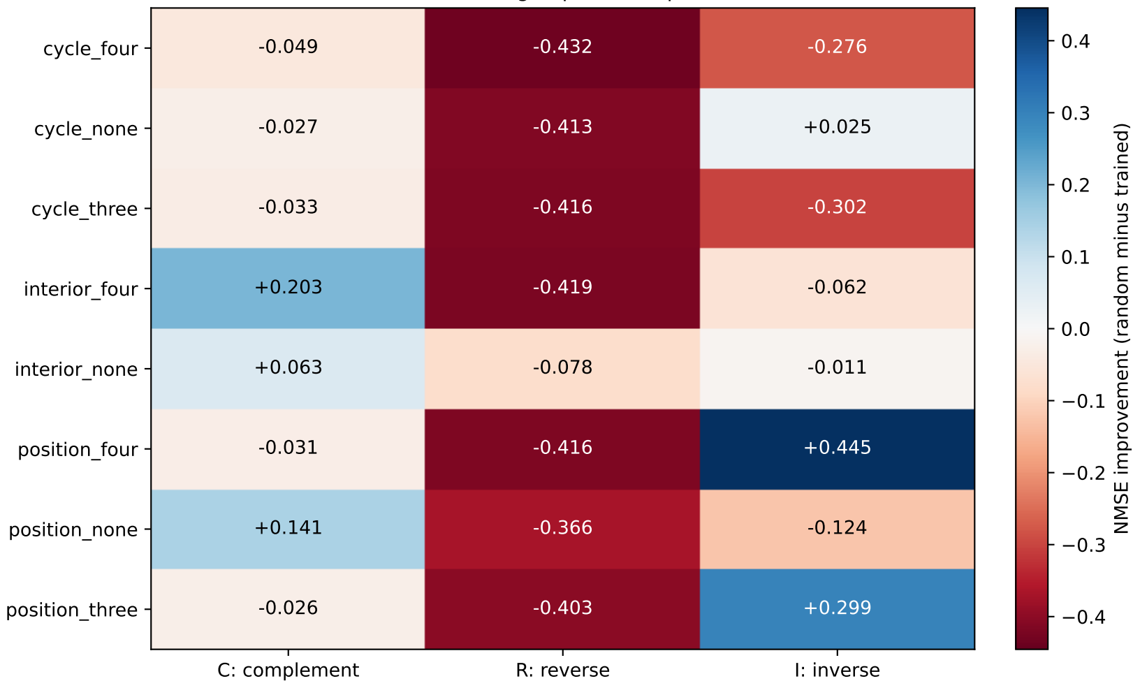
Operator prediction at source queries Positive values: training improves displacement NMSE
