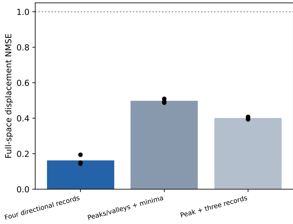
composite nmse
