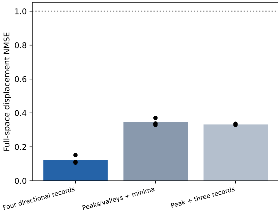
generator nmse
