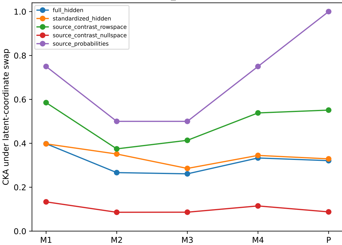
field_symmetry
