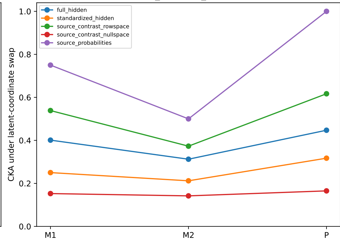
field_matched_support
