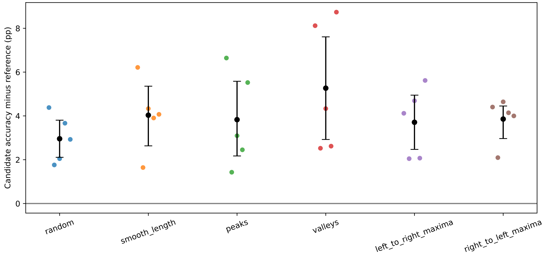
LIS, 256 labels; identical candidate-selected adaptation policy; five new source seeds
