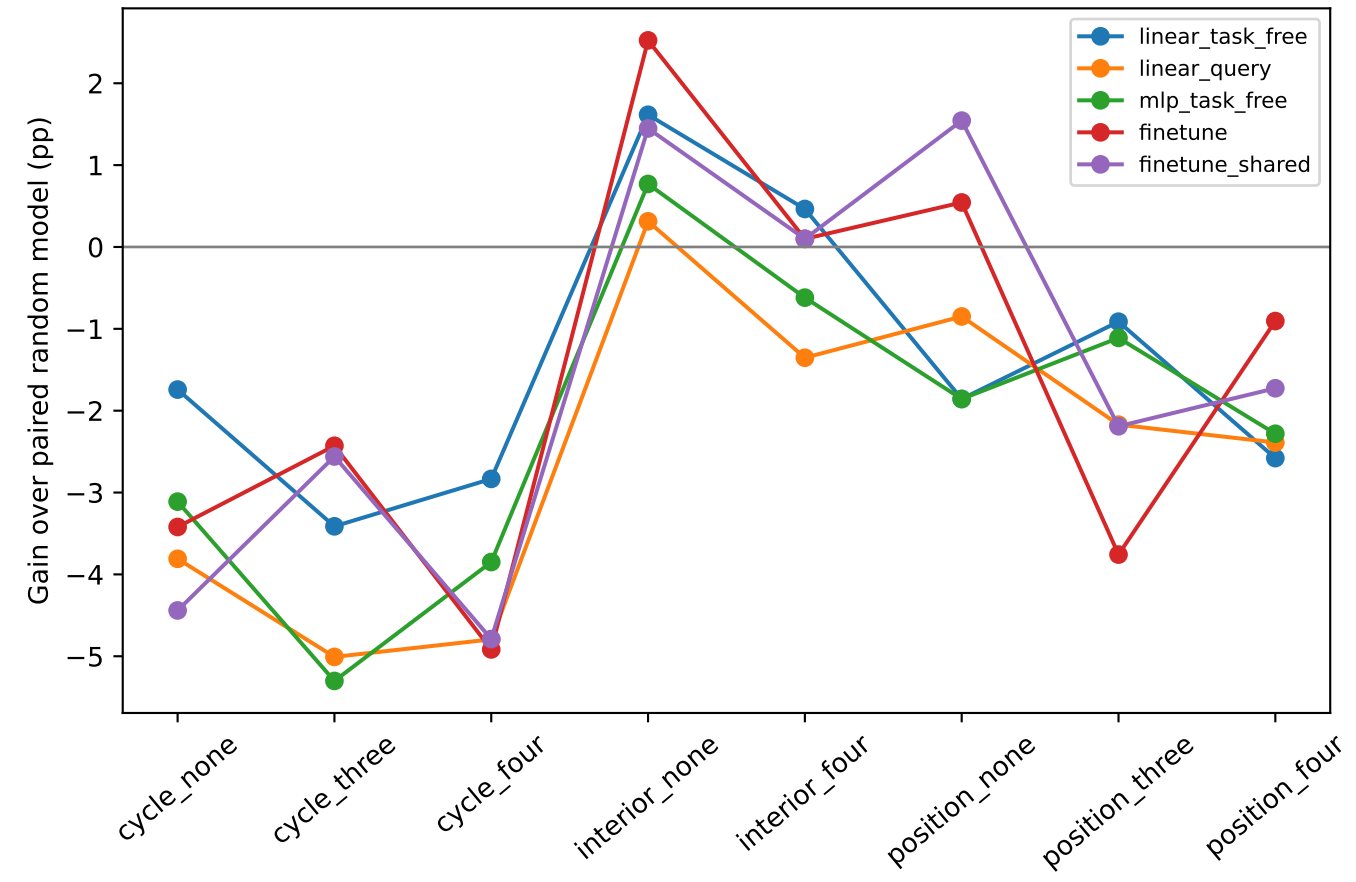
256 target labels
