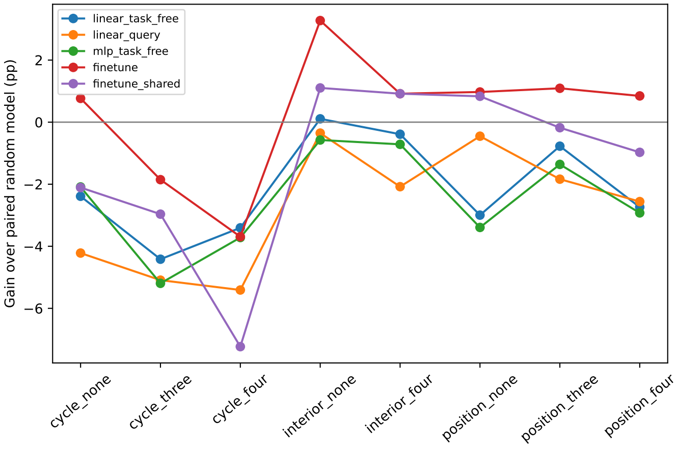
64 target labels
