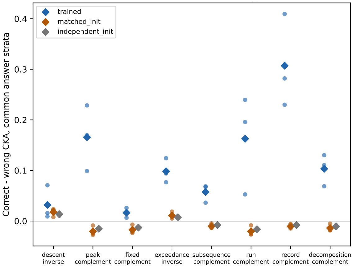
Pooled lengths: task-free ONE_END
