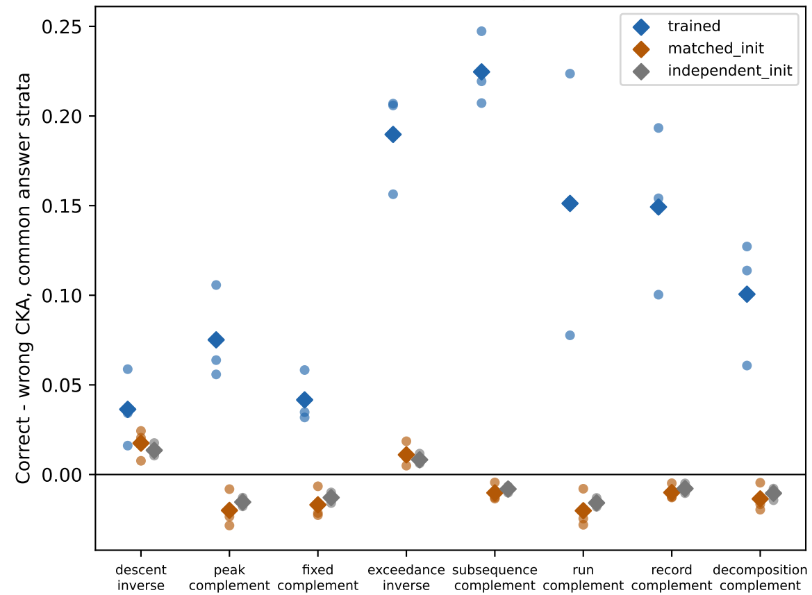
Pooled lengths: task query (=)
