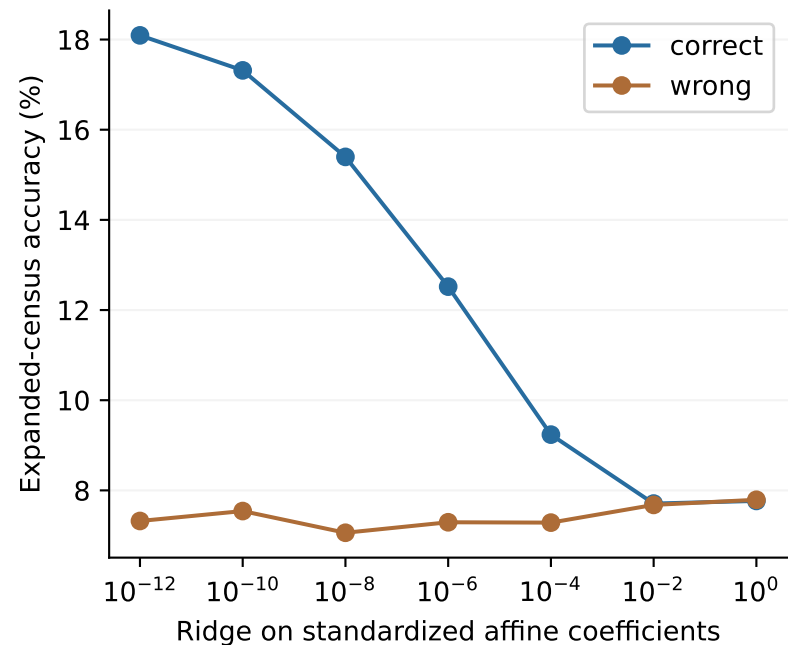
Regularization sensitivity, fixed validation rule
