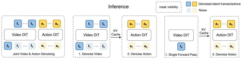
(C) Ours: Action prediction without attending future video. Video prediction only as objective.
