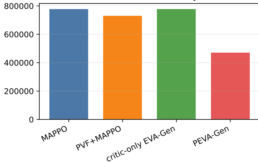
Total communication (bytes)
