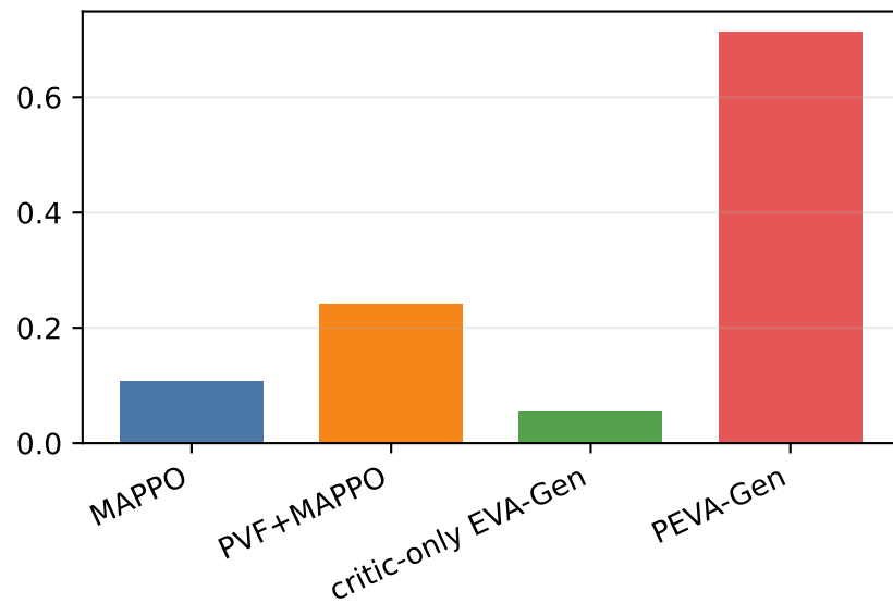
Survival score
