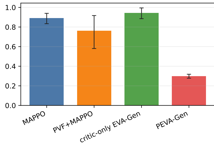
Normalized TTD
