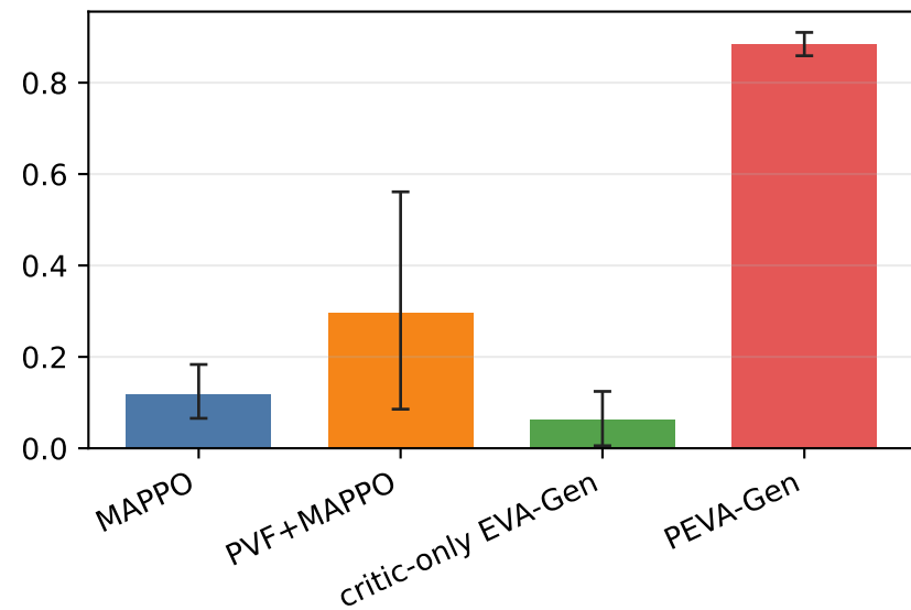
Success rate
