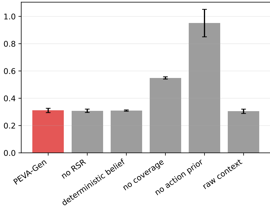
Normalized TTD
