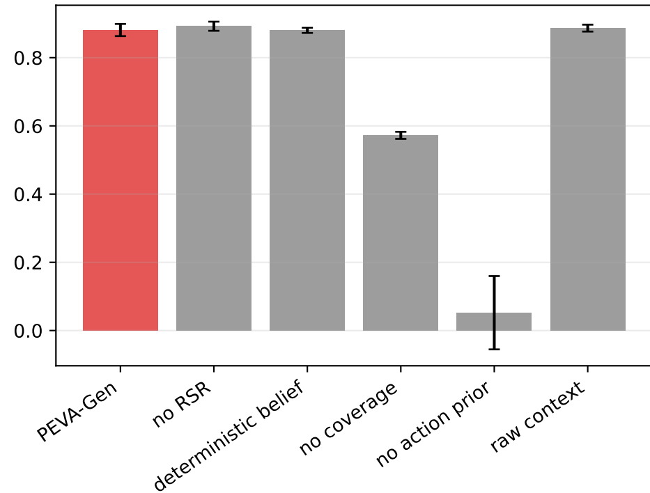
Success rate
