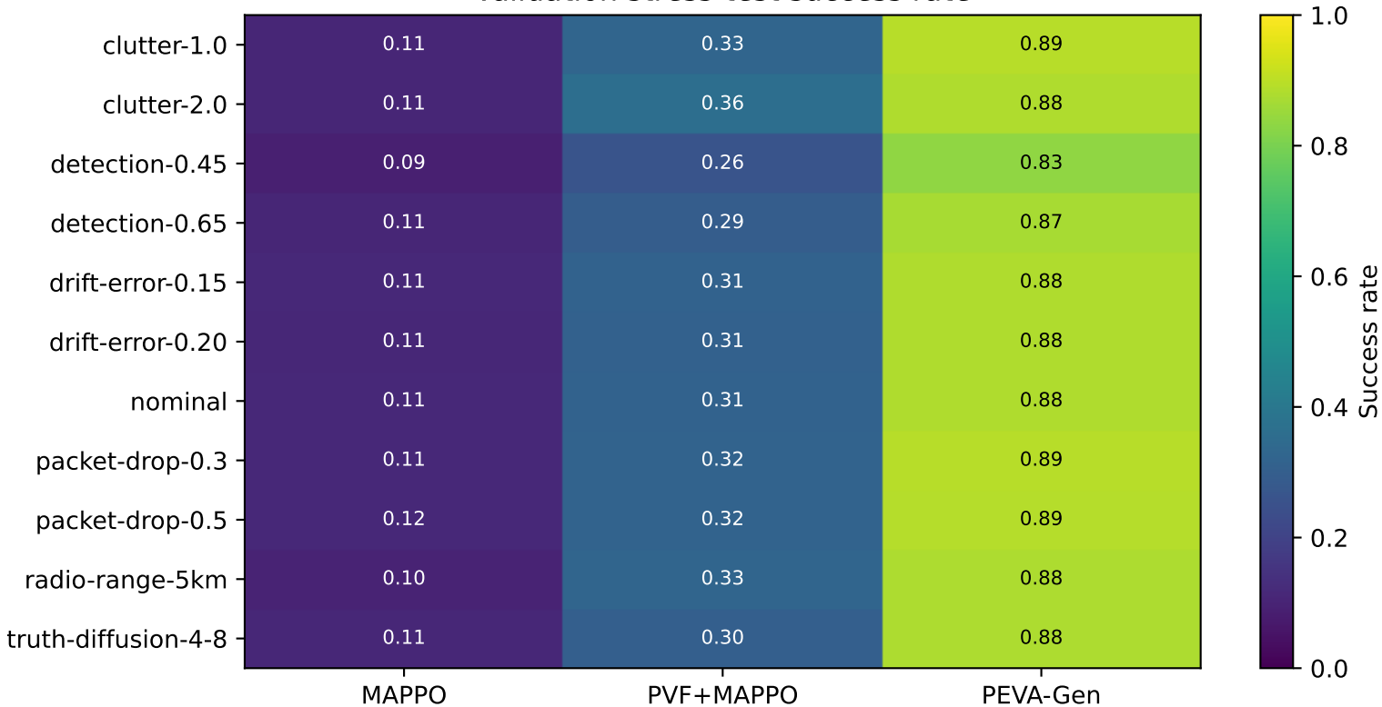
Validation stress-test success rate
