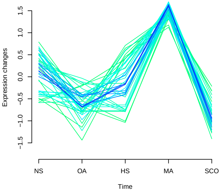
Cluster 5
