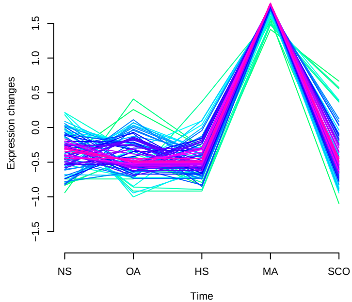
Cluster 6
