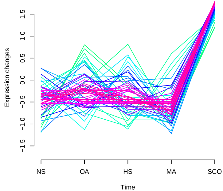
Cluster 4
