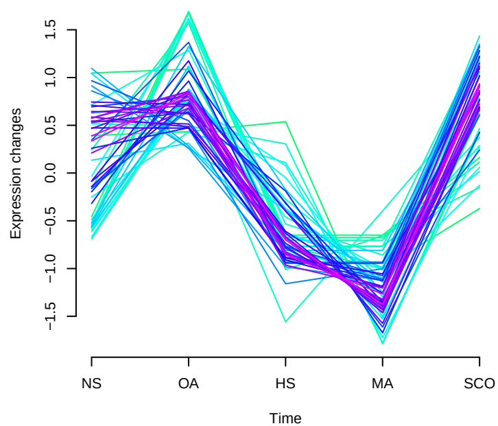
Cluster 6
