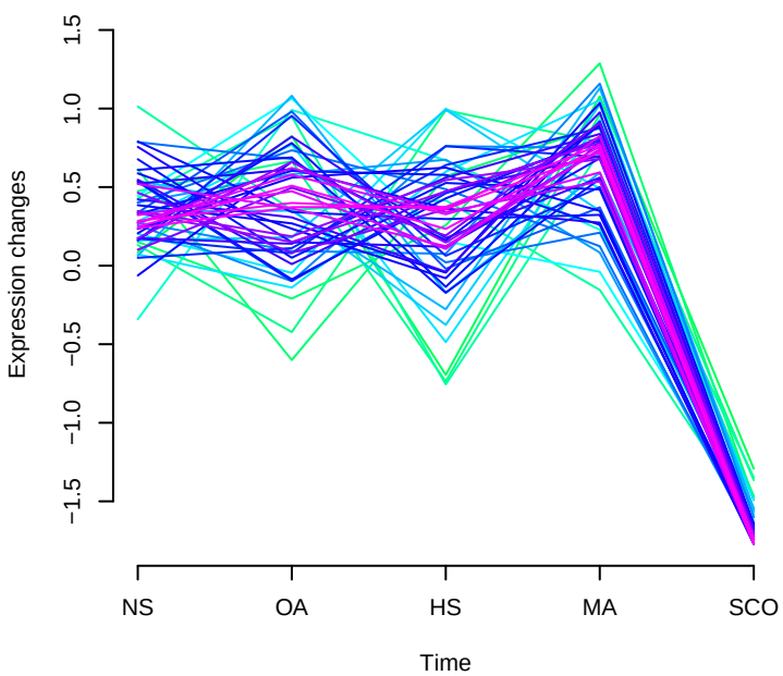
Cluster 3
