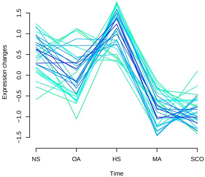
Cluster 5
