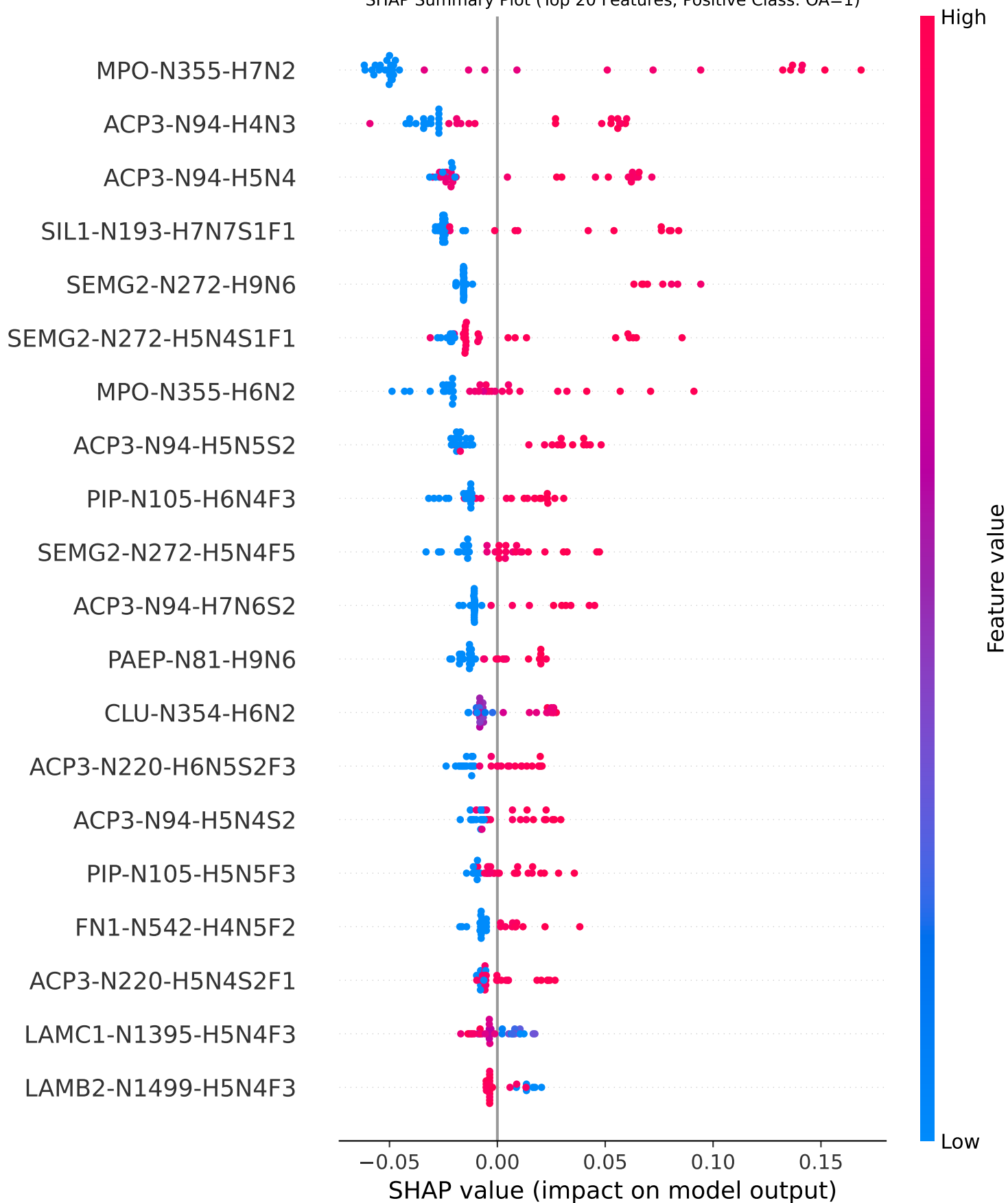
SHAP Summary Plot (Top 20 Features, Positive Class: OA=1)
