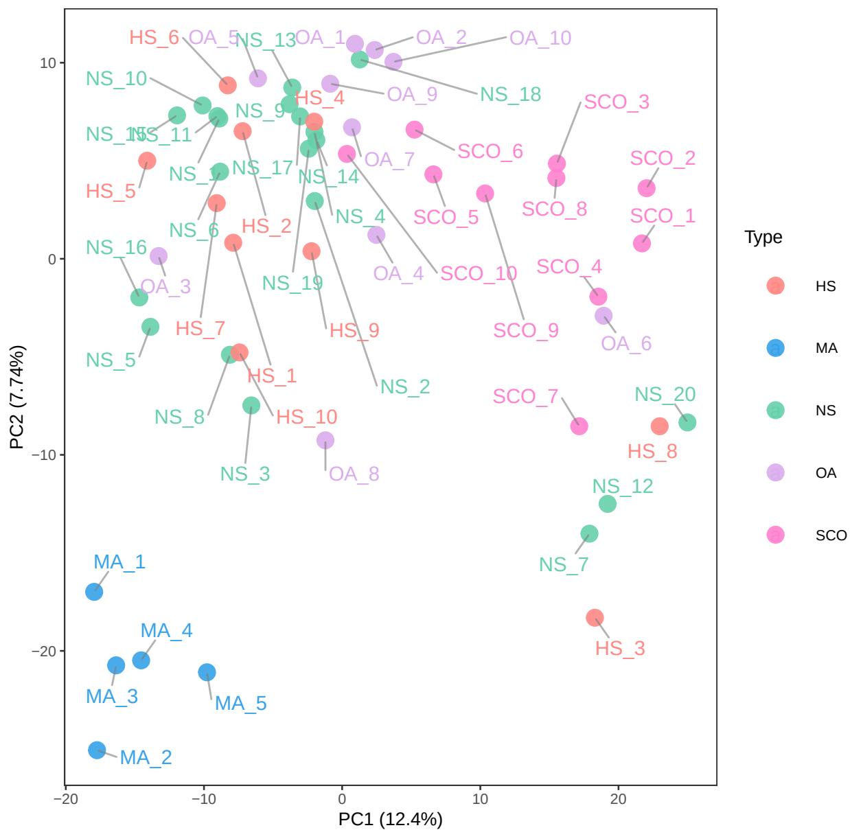
PCA Analysis – Colored by Type
