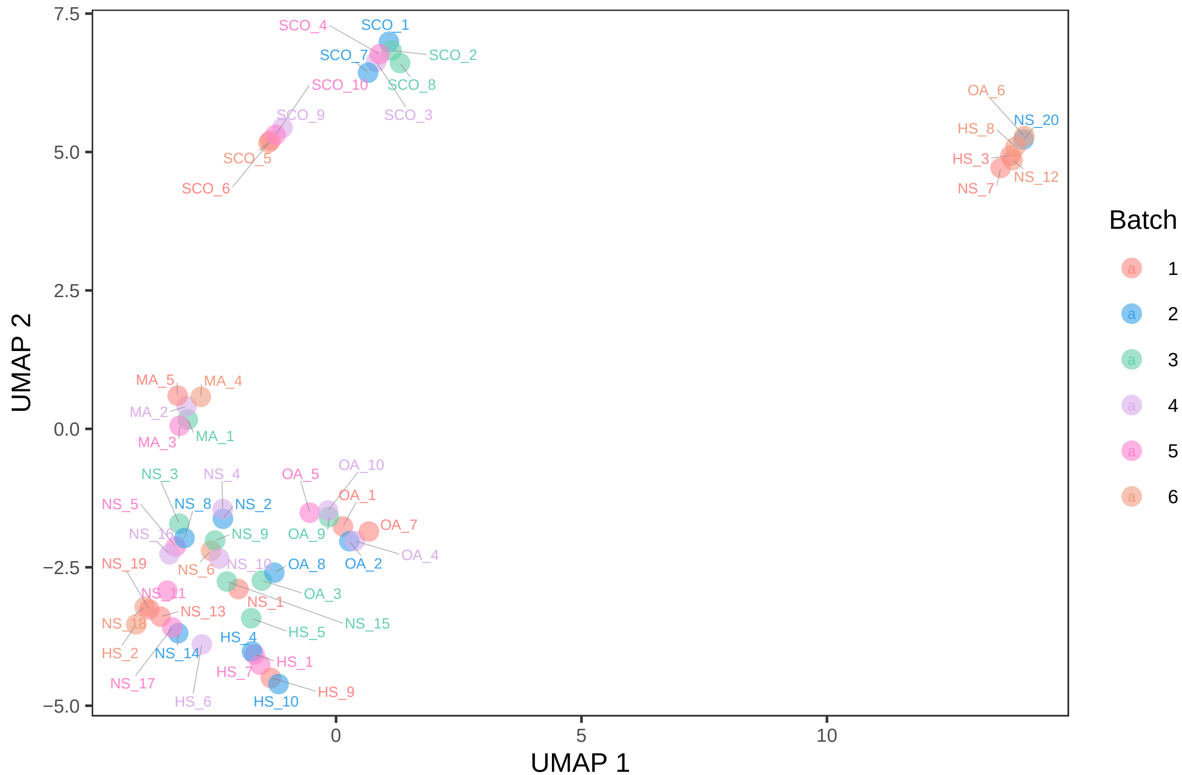
UMAP Analysis – Colored by Batch
