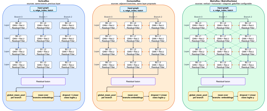
Figure 1. Architecture overview of the compared residual neighborhoods on the branch-by-layer grid. The same message-passing backbone and graph-level readout are kept fixed while the residual routes are changed.
