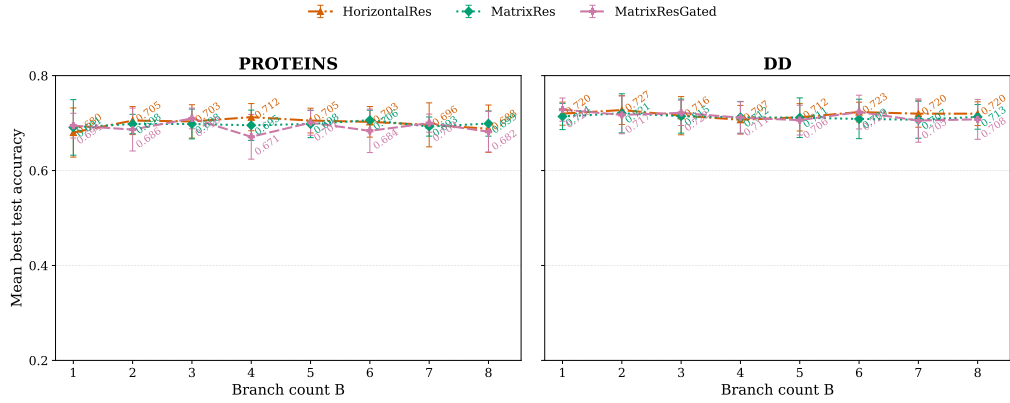
Figure 5. Branch-count ablation for HorizontalRes, MatrixRes, and MatrixResGated on PROTEINS and DD under GCNConv. The best branch budget is dataset- and topology-dependent.
