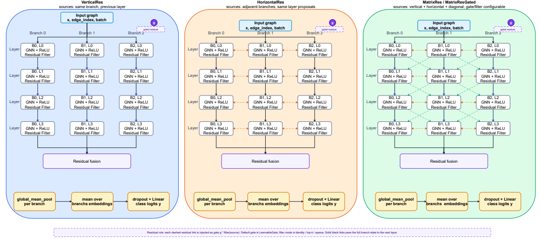
Figure 1. Architecture overview of the compared residual neighborhoods on the branch-by-layer grid. The same message-passing backbone and graph-level readout are kept fixed while the residual routes are changed.
