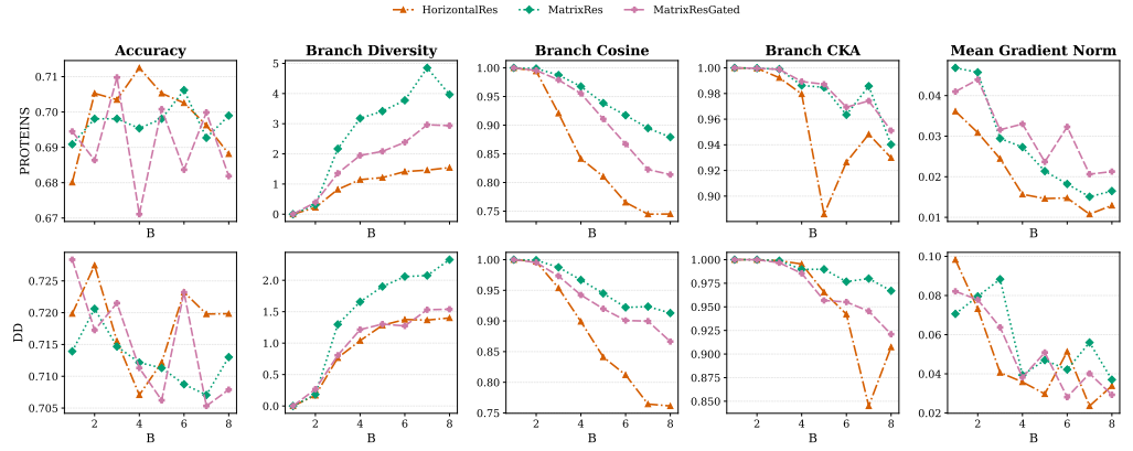
Figure 6. Mechanism summary linking branch-count accuracy to branch diversity, branch cosine similarity, branch CKA, and mean gradient norm.
