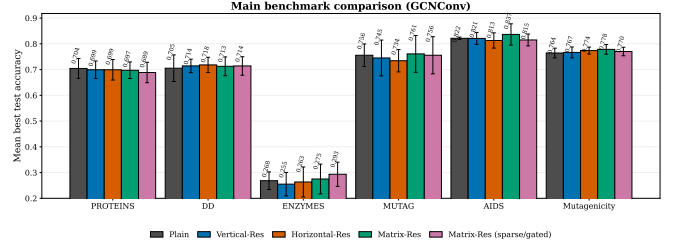
Fig. 3. GCNConv benchmark at B = 3 . Bars show five-fold mean best test accuracy with fold-level standard-deviation error bars.
