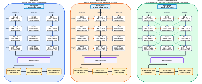
Fig. 1. Architecture overview of the compared residual neighborhoods on the branch-by-layer grid. The same message-passing backbone and graph-level readout are kept fixed while the residual routes are changed.
