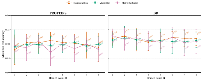
Fig. 5. Branch-count ablation for HorizontalRes, MatrixRes, and MatrixResGated on PROTEINS and DD under GCNConv. The curves are not monotonic: accuracy improves only within an effective operating region before saturating or declining.
