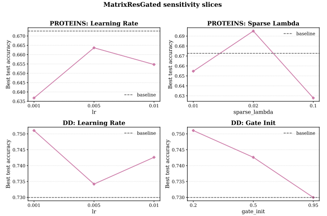
Fig. 7. Fold-0 MatrixResGated sensitivity scan at B = 3 . The scan identifies candidate operating regions but is not treated as final hyperparameter evidence.
