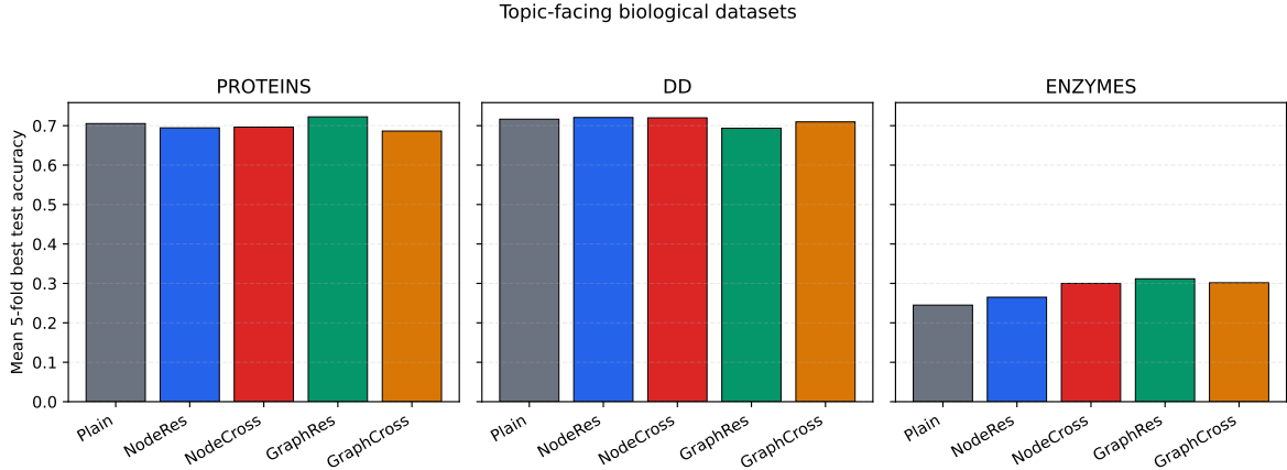
Figure 6: Focused comparison on the topic-facing datasets PROTEINS, DD, and ENZYMES. The pattern is mixed rather than one-sided: graph-level residual refinement is strongest on PROTEINS and ENZYMES, while DD favors node-level reuse, with NodeCrossGNN remaining competitive but not dominant.
