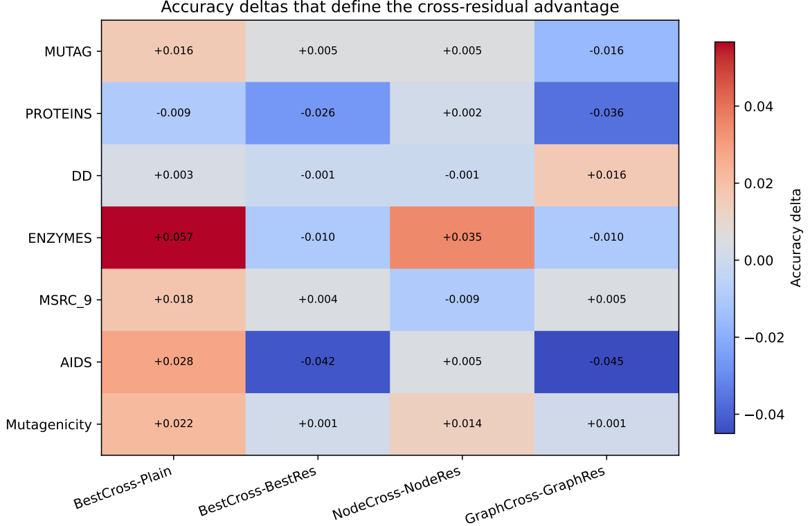
Figure 4: Accuracy deltas that define the practical value of cross-residual routing. Positive values indicate an advantage for the cross design, while negative values indicate that the corresponding plain or residual alternative remains stronger.
