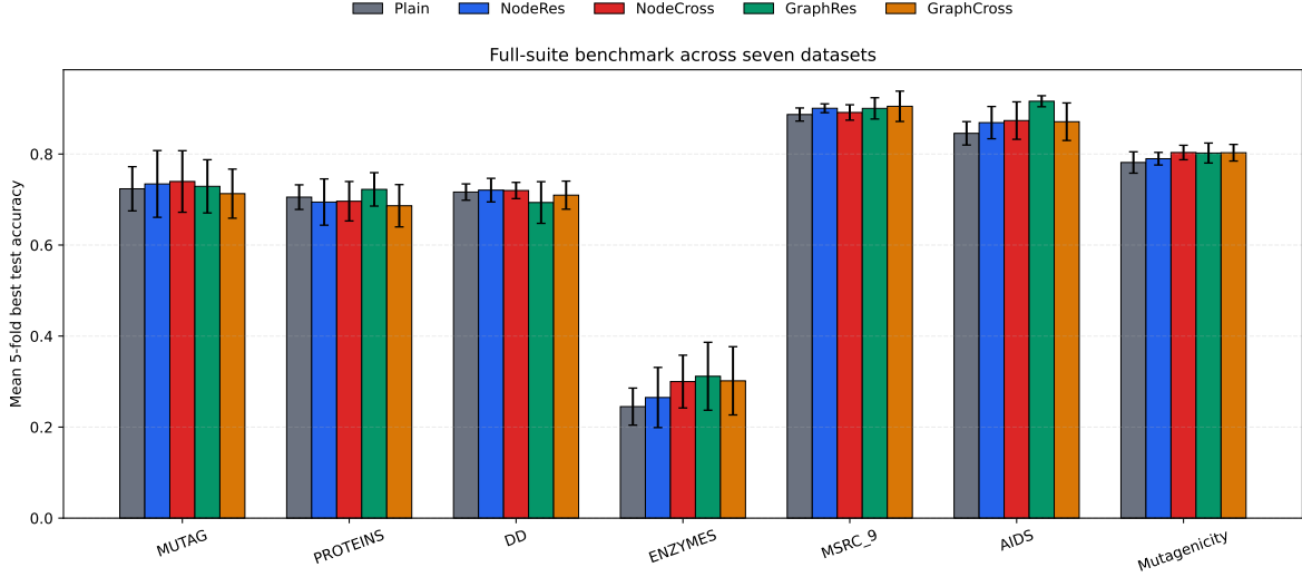
Figure 3: Full-suite benchmark over all seven datasets. Each bar reports mean 5-fold best test accuracy, and error bars show the fold-level standard deviation. The figure makes the winner pattern visually explicit: residual variants dominate on PROTEINS, DD, ENZYMES, and AIDS, while cross variants win on MUTAG, MSRC_9, and Mutagenicity.
