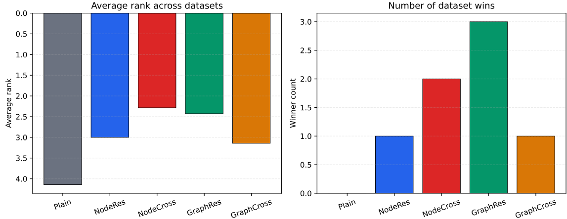
Figure 5: Aggregate ranking signals across the complete suite. The left panel reports average rank, where smaller is better. The right panel reports dataset winner counts. NodeCrossGNN has the best average rank, but GraphResGNN has the largest number of outright wins, which explains why residual reuse remains the stronger default family in the final narrative.
