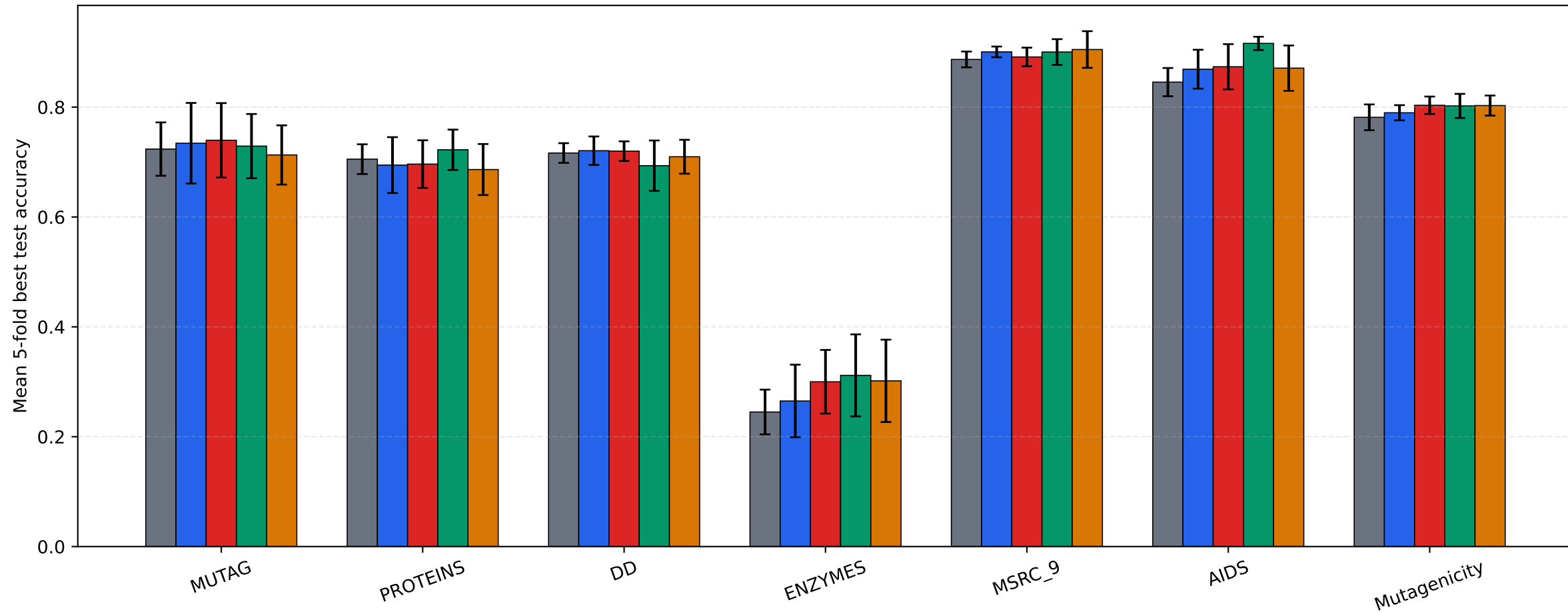
Full-suite benchmark across seven datasets
