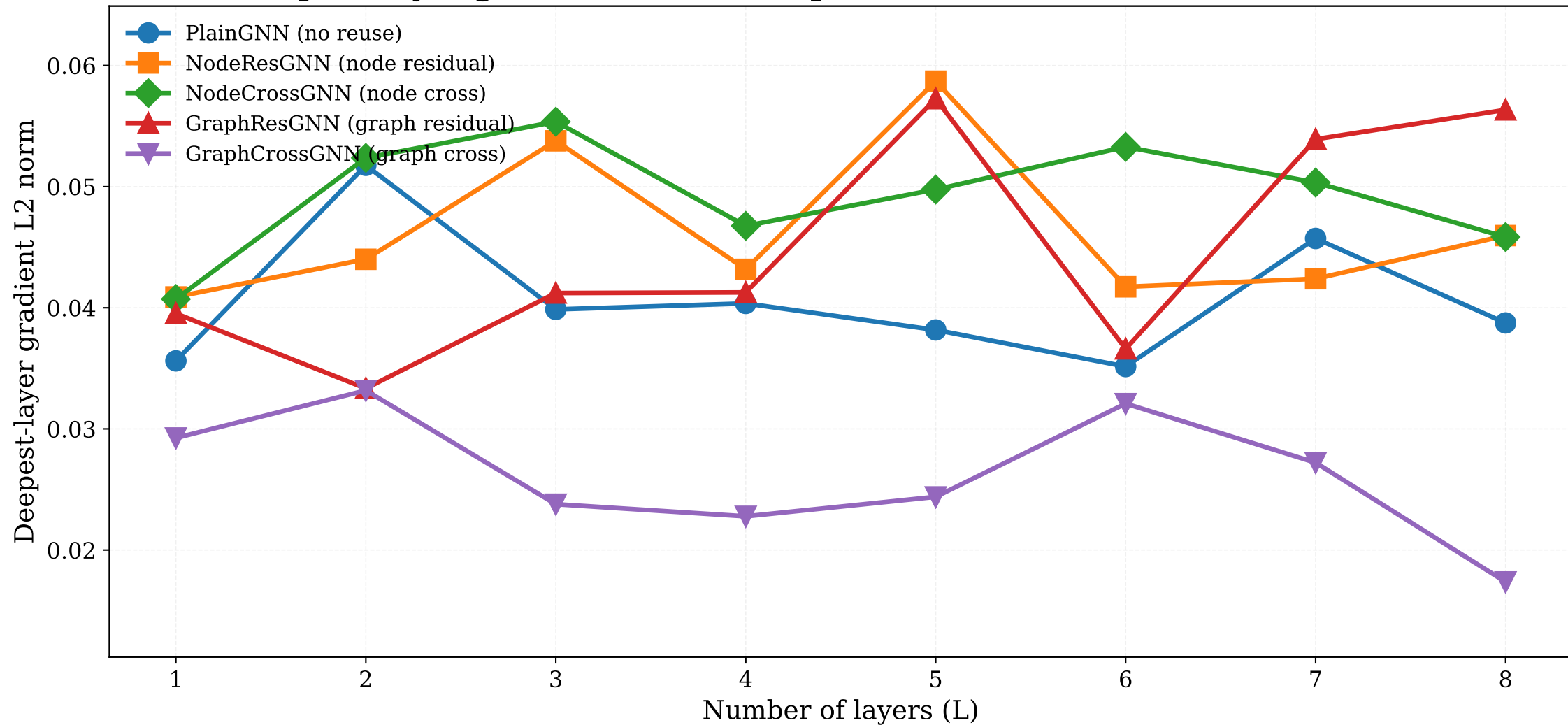
Deepest-layer gradient norm vs depth (L=1--8) — PROTEINS (GCNConv)
