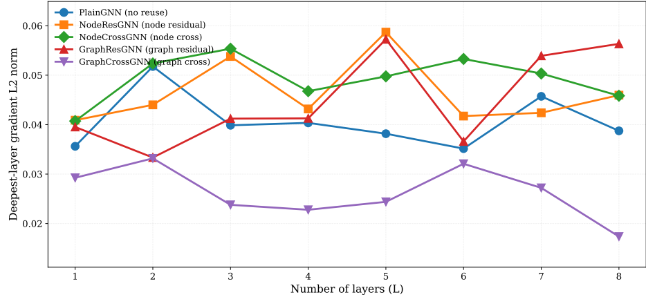
Deepest-layer gradient norm vs depth ( L=1\text{--}8 ) — PROTEINS (GCNConv)
