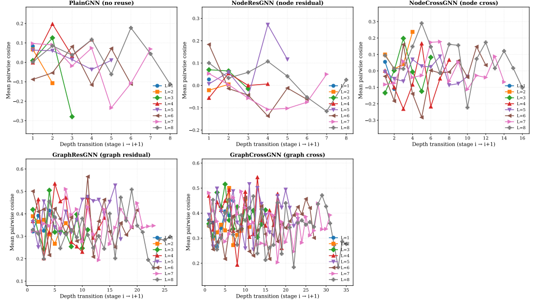
Figure 4. Cosine similarity between adjacent depth stages across L = 1\text{--}8 .
