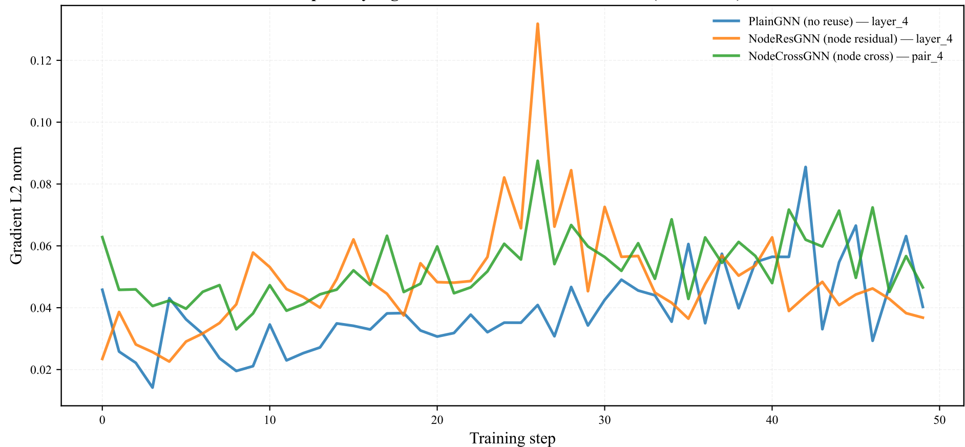
Deepest-layer gradient evolution — PROTEINS (GCNConv)
