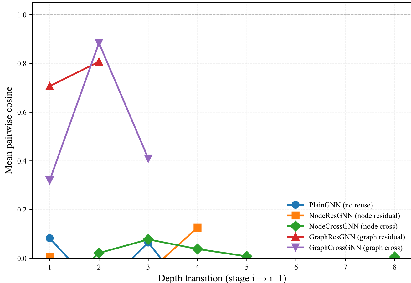
Cosine similarity between adjacent depth stages
