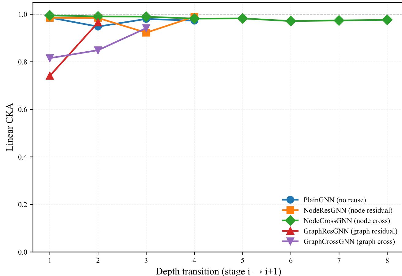
CKA similarity between adjacent depth stages
