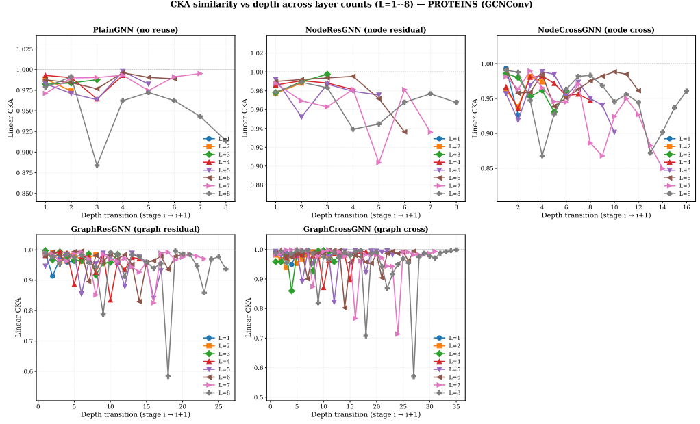
Figure 6. CKA similarity between adjacent depth stages across L = 1-8 on PROTEINS under GCNConv.
