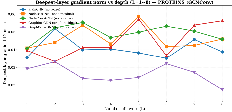
Figure 7. Deepest-layer gradient L2 norm across L = 1-8 (PROTEINS, GCNConv).
