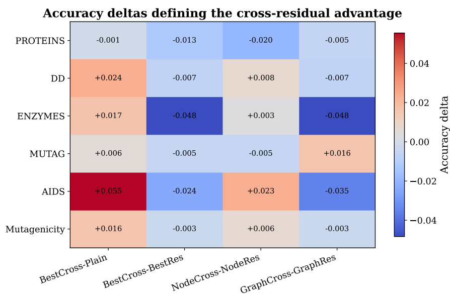
Figure 5. V3 cross-residual advantage heatmap. Positive cells indicate that the best cross-residual variant outperforms the indicated comparator on that dataset.
