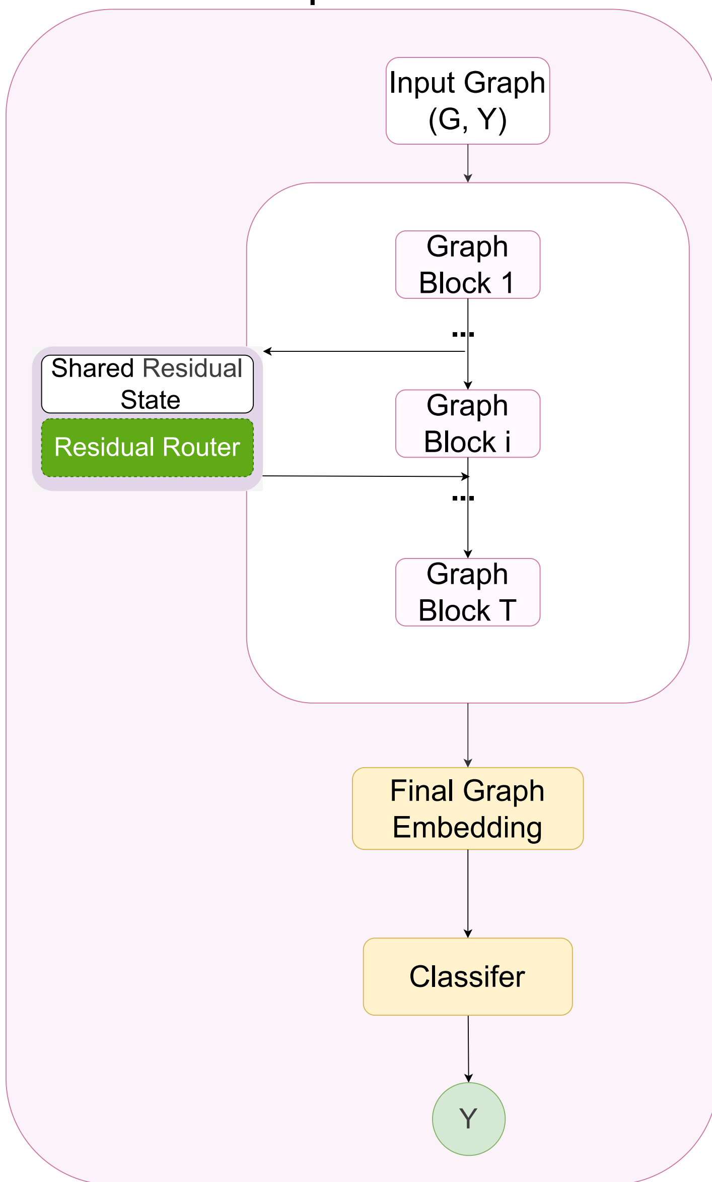
GraphResGNN
