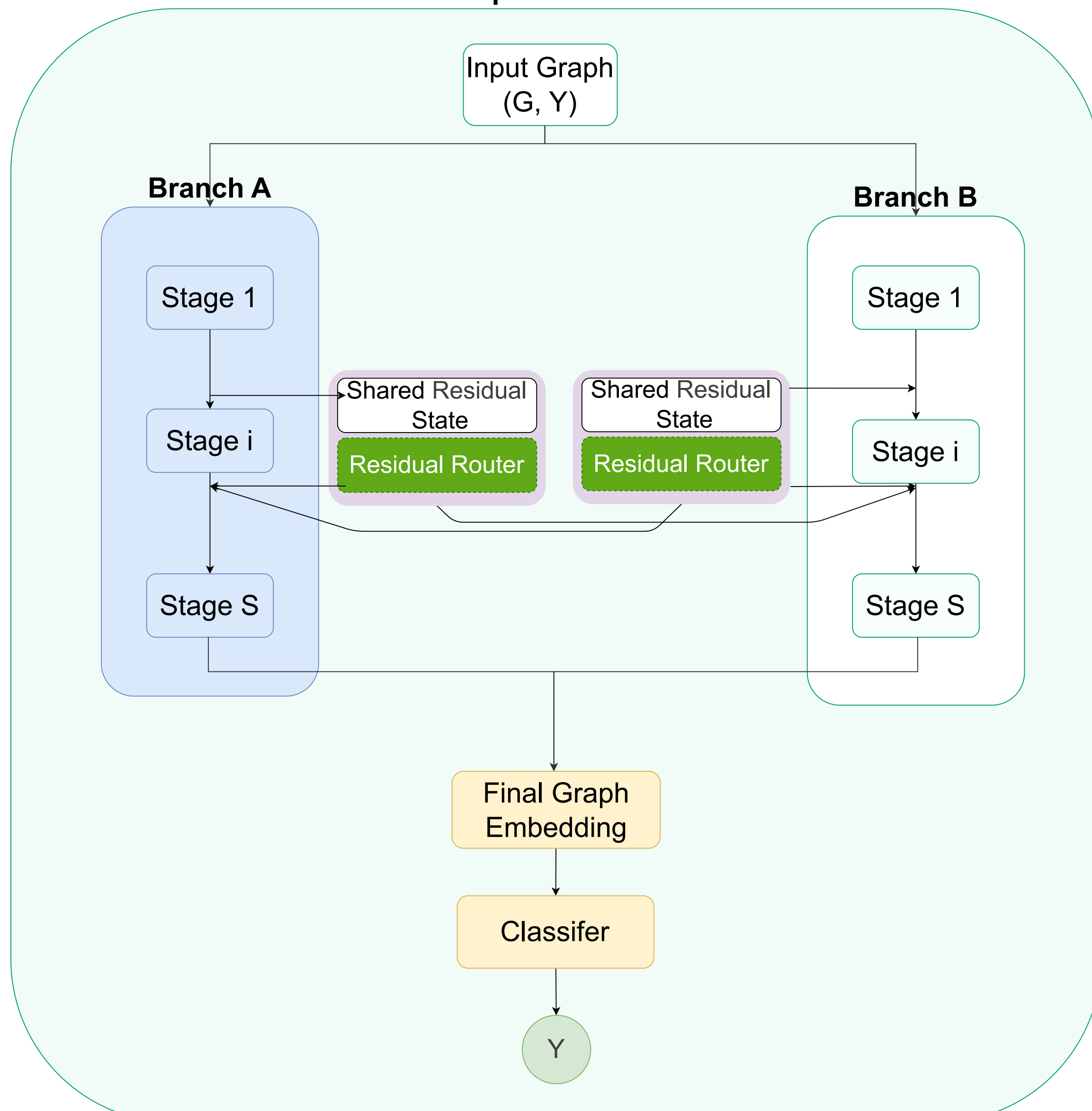
GraphCrossGNN
