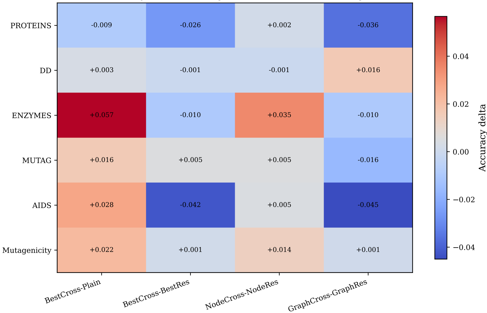
Accuracy deltas defining the cross-residual advantage
