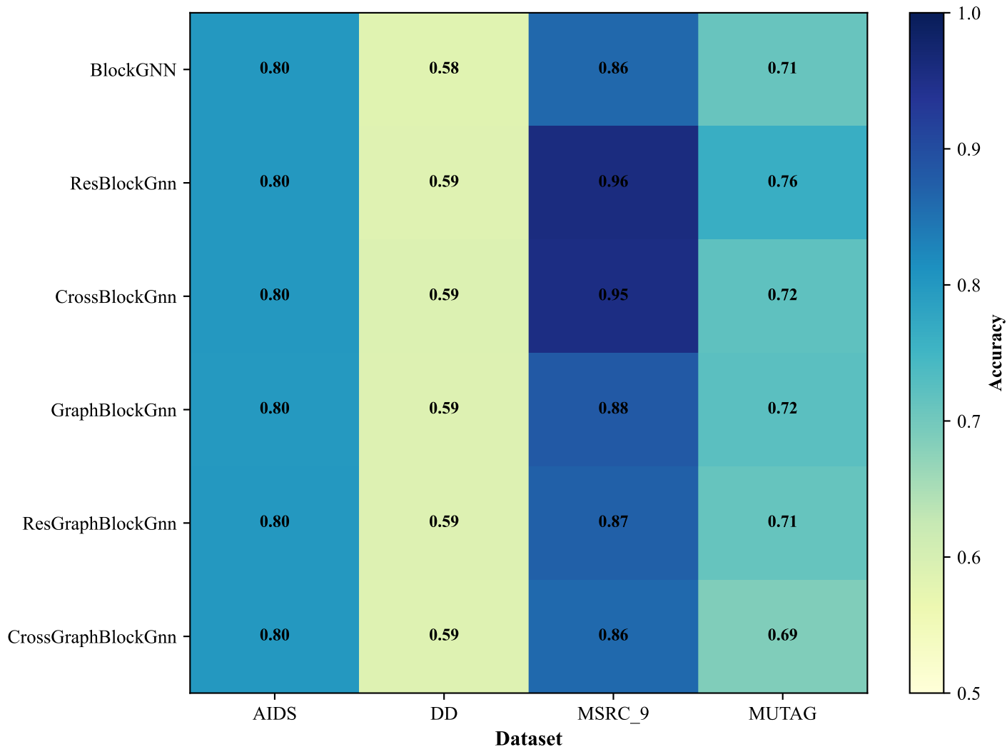
Model Performance Heatmap (Mean Accuracy)
