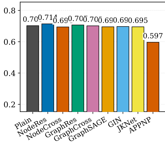
Mean 5-fold best test accuracy
