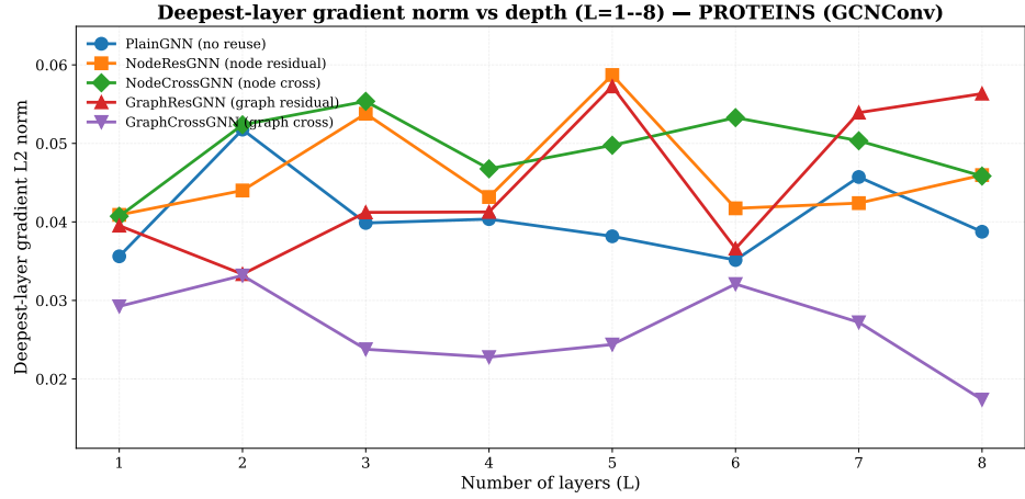
Figure 5. Deepest-layer gradient L2 norm across L = 1-8 (PROTEINS, GCNConv).
