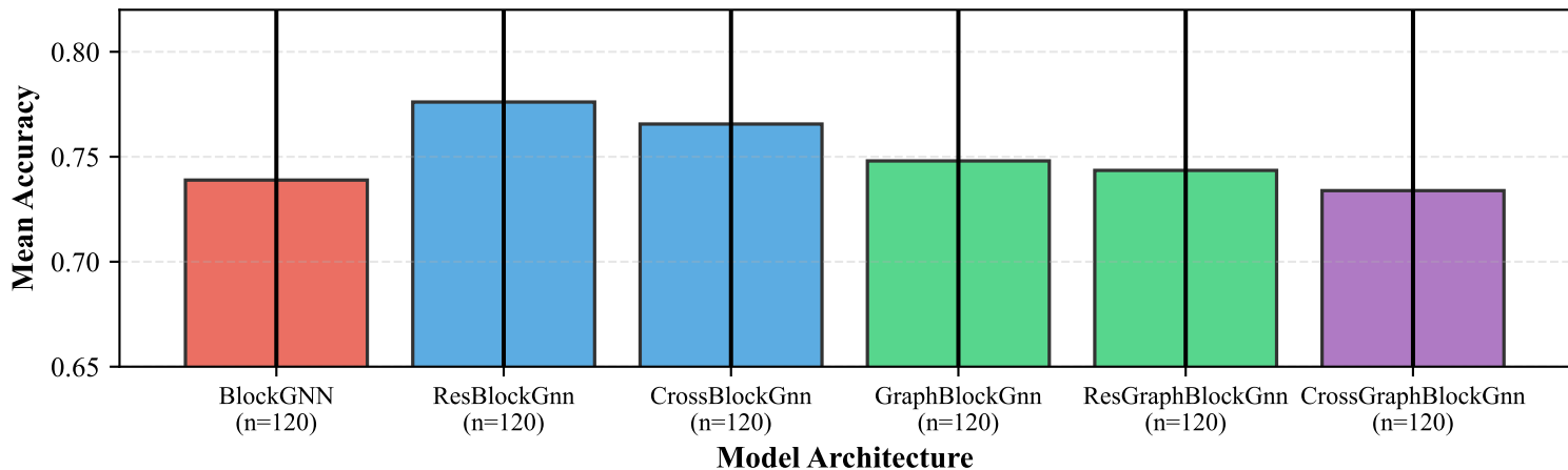
Average Performance Across All Datasets
