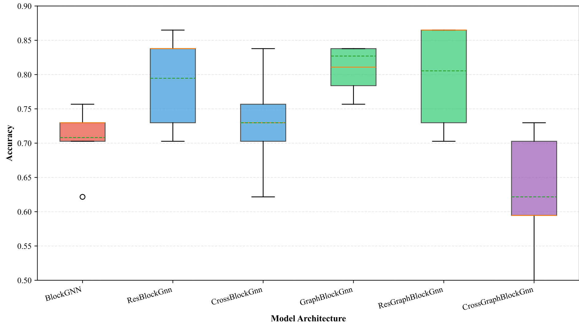
5-Fold CV Distribution on MUTAG (GCN, h=2, dim=32)
