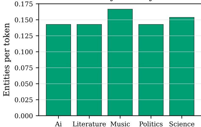
Entity density
