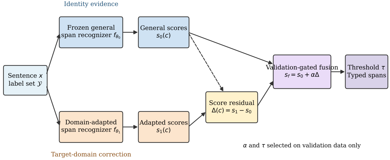
Figure 1: Gated score-residual adaptation. Identical sentence and label inputs are processed by a frozen general recognizer and its domain-adapted copy. Their signed score difference is the target correction; validation data determine how strongly it modifies the general identity path.
