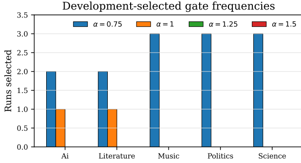
Figure 8: Frequency of development-selected residual coefficients across three runs.
