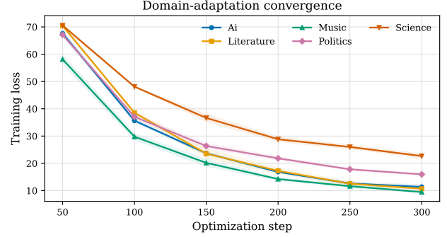
Figure 10: Mean recorded training loss by target domain; shading denotes one sample standard deviation across three runs.
