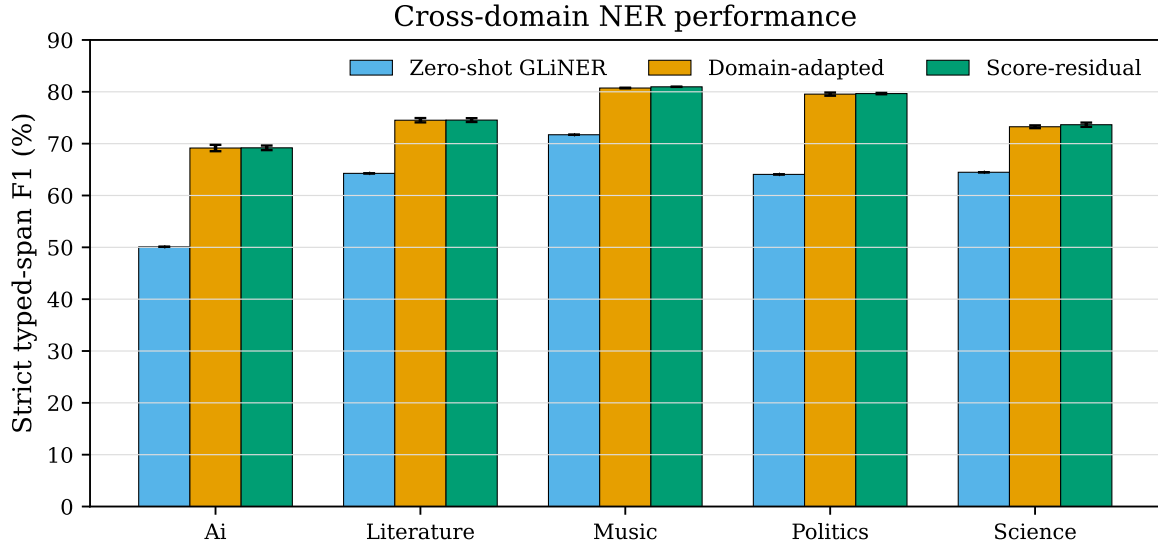
Figure 6: Strict typed-span F1 for the frozen general, domain-adapted, and score-residual configurations.
