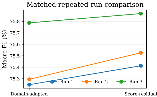
Figure 7: Matched domain-macro F1 before and after score-residual fusion for the three independent runs.
