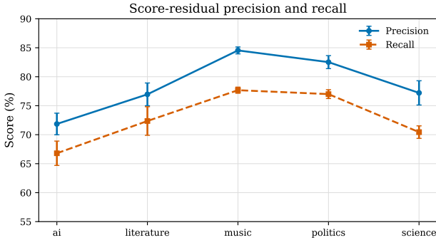
Figure 9: Precision and recall of the score-residual model by domain.
