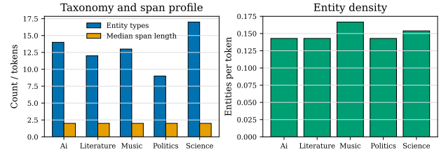
Figure 4: Entity taxonomy, span-length, and density profile computed from official CrossNER annotations.
