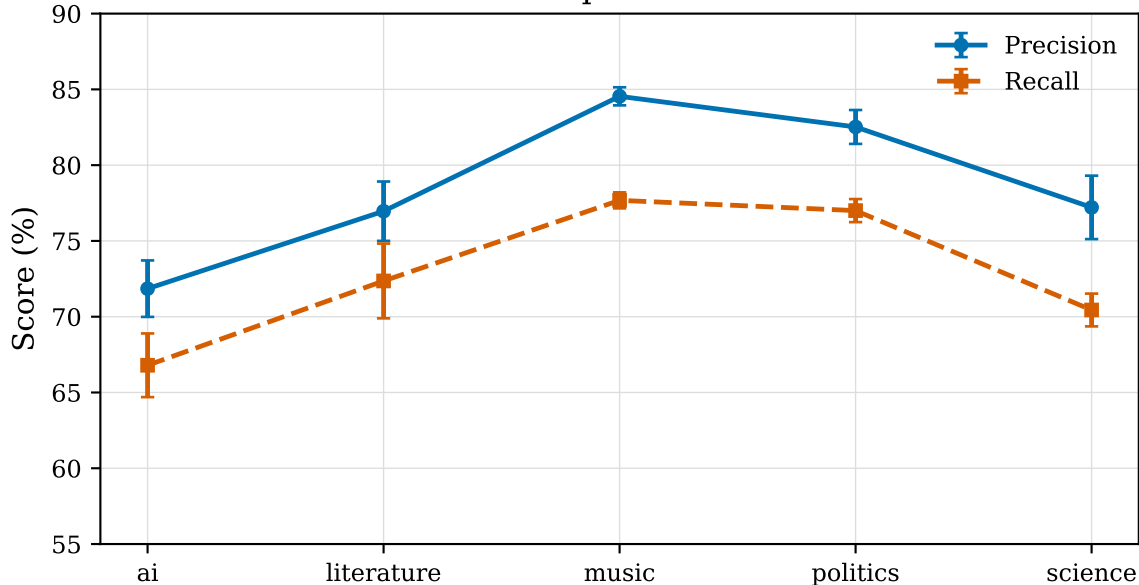
Score-residual precision and recall
