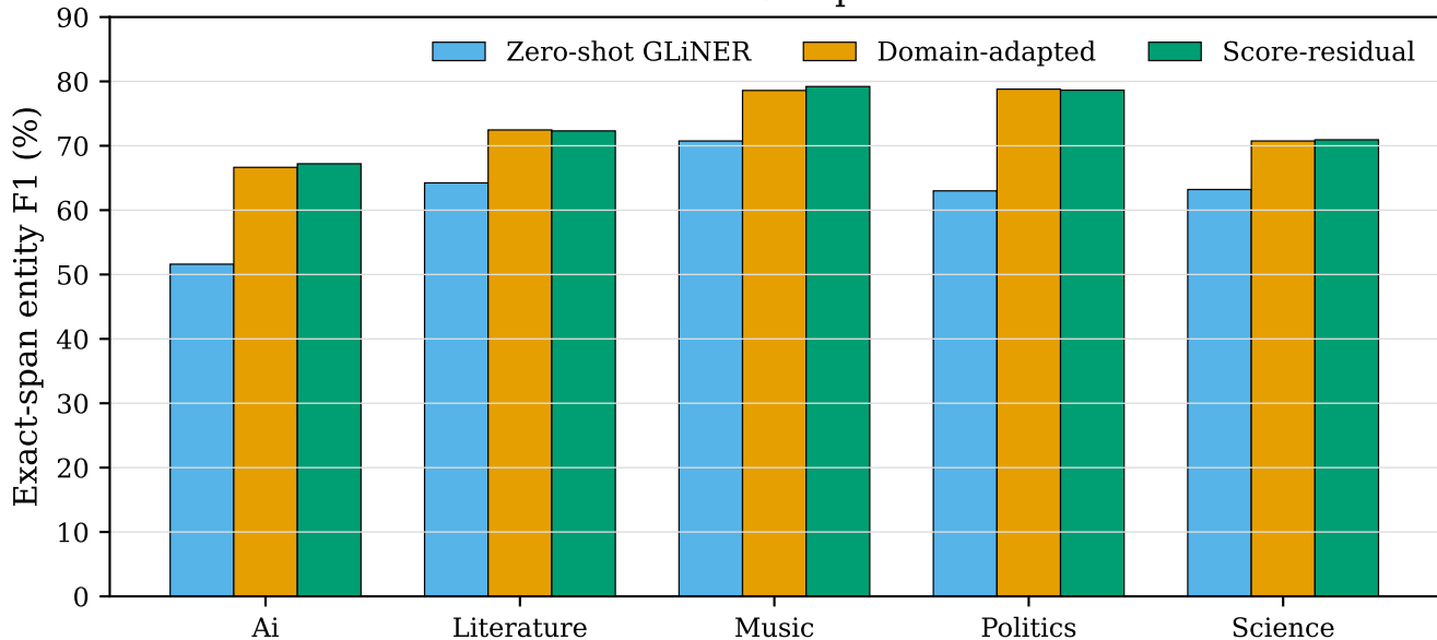
Cross-domain NER performance
