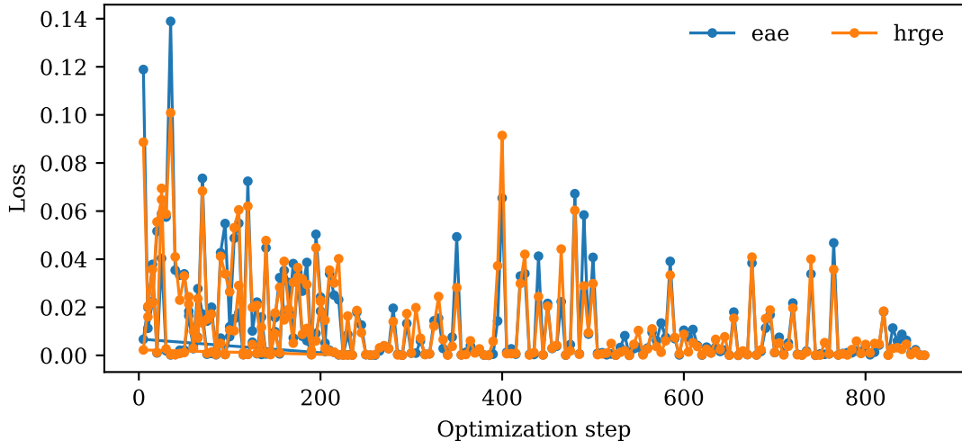
Training-loss diagnostic (committed pilot run)
