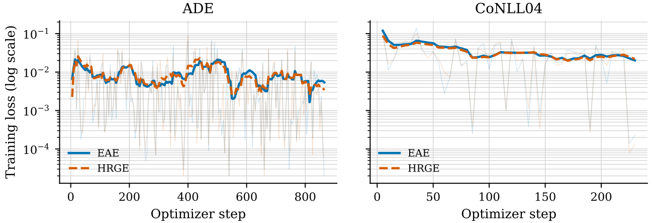
Figure 4: Audited seed-42 training loss for the EAE and HRGE adapters. Raw observations (faint) were written to runner stdout every five optimizer steps; emphasized curves are ten-observation trailing means. The logarithmic scale retains the large variation in the raw observations. No intermediate values are reconstructed or interpolated.
