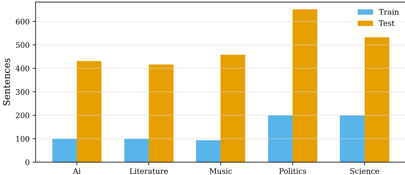
CrossNER domain distribution
