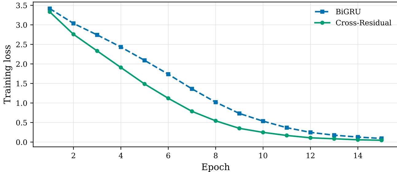
Optimization behavior on CrossNER-Science
