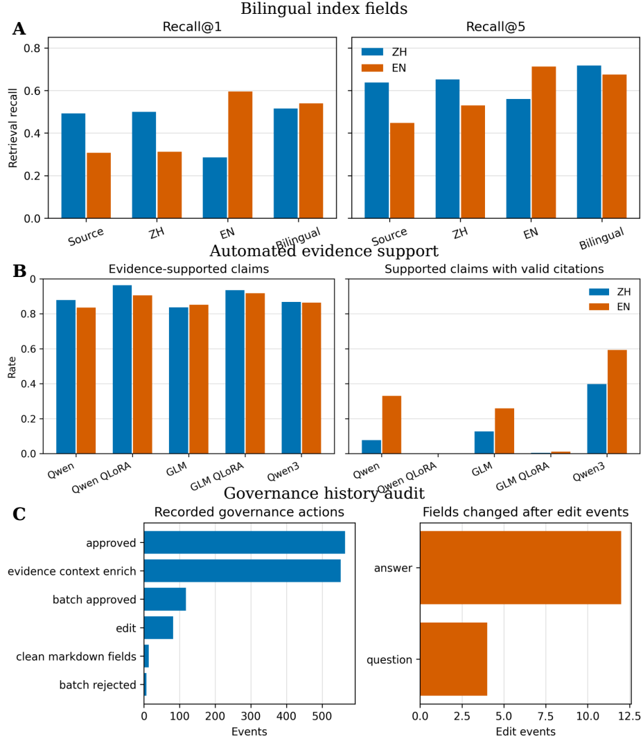
Figure 5: Three validation layers. Panel A compares source-only, Chinese-field, English-field and bilingual indexes; Panel B compares semantic support against retrieved and explicitly cited evidence; Panel C audits immutable review events and before-state snapshots. Together the panels show retrieval balance, evidence support and governance traceability without reducing them to one score. An em dash indicates that a measure is not language-specific.
