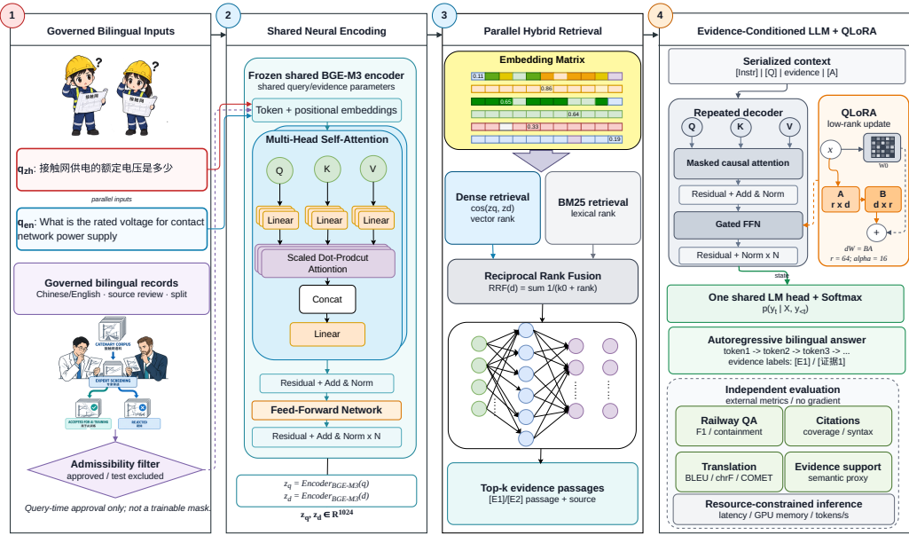
Figure 1: Bilingual railway QA workflow from left to right: governed bilingual input, shared encoding, lexical and dense retrieval, fusion, evidence-conditioned generation and evaluation. The rightmost module shows the QLoRA adapter path alongside the frozen base model.
