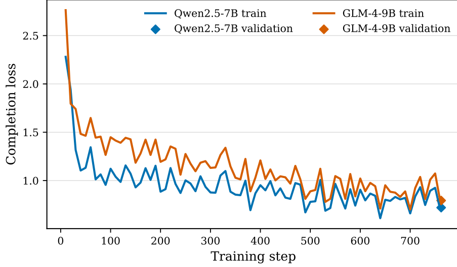
Figure 3: Completion-only QLoRA optimisation for Qwen2.5-7B and GLM-4-9B. Lines show logged training loss; diamonds mark the end-of-epoch validation measurement for each model. Source: Authors’ own work.
