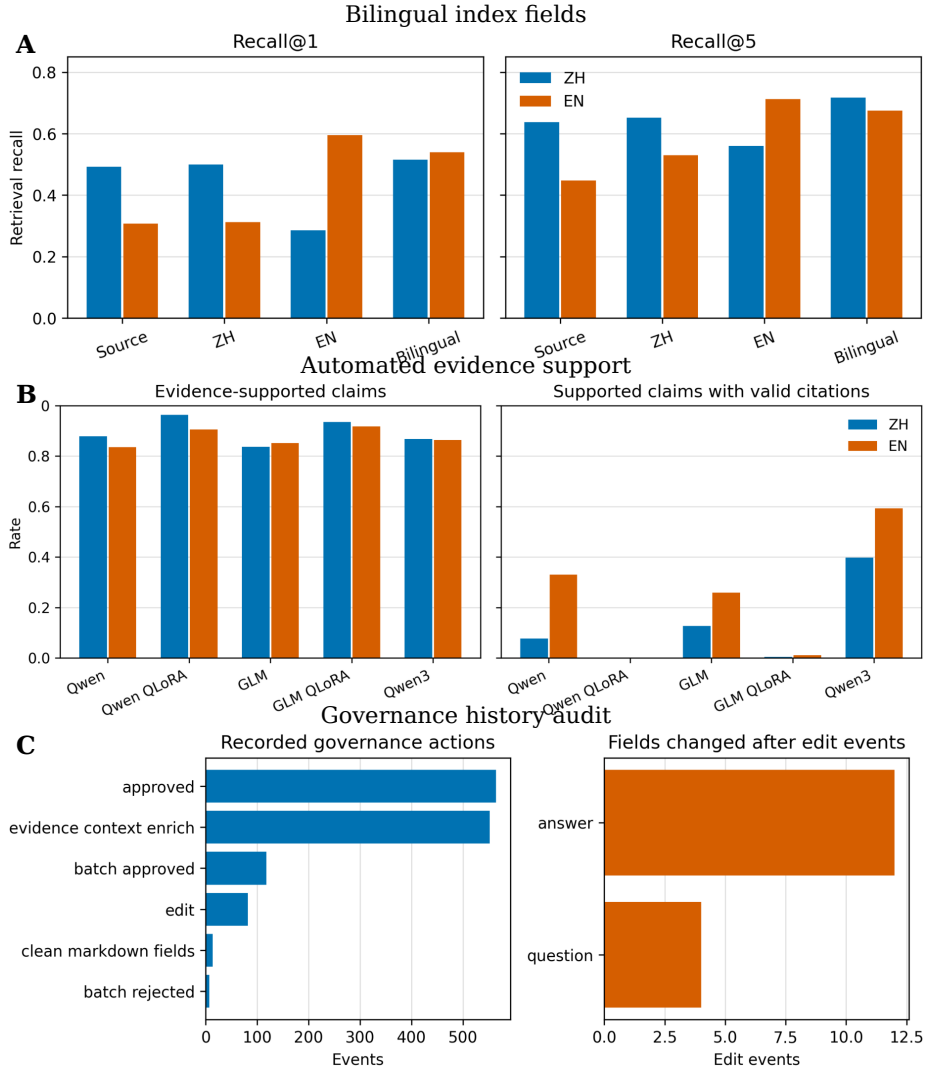
Figure 5: Three validation checks. Panel A compares source-only, Chinese-field, English-field and bilingual indexes; Panel B compares semantic support against retrieved and explicitly cited evidence; Panel C audits immutable review events and before-state snapshots. An em dash indicates that a measure is not language-specific.
