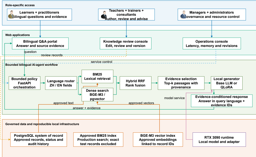
Figure 1: Four-layer bounded bilingual agent workflow linking three role-access clusters to Web applications, governed retrieval, local generation and single-workstation infrastructure. Solid arrows denote runtime data flow; dashed arrows denote governance or control. Source: Authors’ own work.
