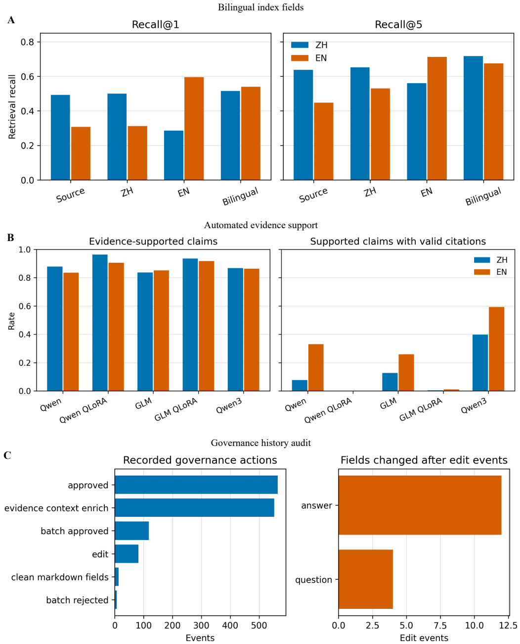
Figure 8: Bilingual index, automated evidence support and governance-history validation. Panels A-C report field ablation, evidence support and governance audit results, respectively. Source: Authors' own work.
