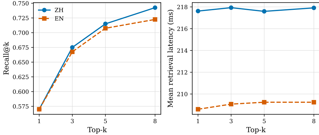
Figure 3: Hybrid evidence-equivalent retrieval quality and latency across top-k settings. Left: Evidence Recall@k; right: mean retrieval latency. Source: Authors’ own work.
