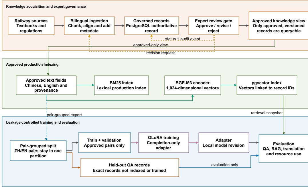
Figure 2: Expert-governed knowledge, production-index and evaluation lifecycle with exact held-out records excluded from indexing and training. Source: Authors’ own work.
