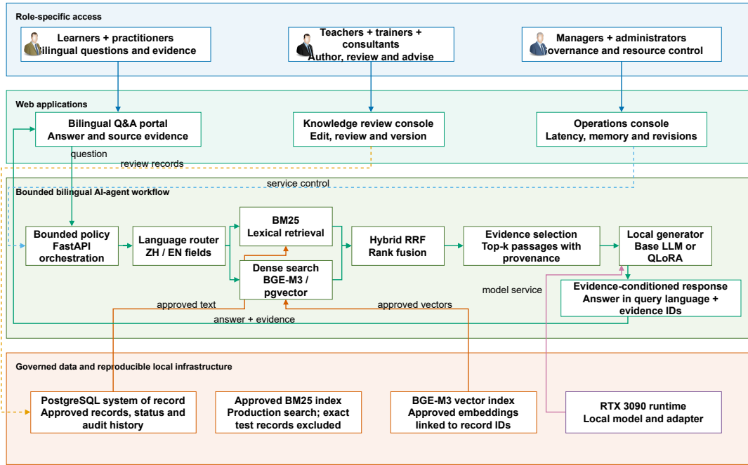
Figure 1: Four-layer bounded bilingual agent workflow linking three role-access clusters to Web applications, governed retrieval, local generation and single-workstation infrastructure. Solid arrows denote runtime or data flow; dashed arrows denote governance or control. Source: Authors’ own work.
