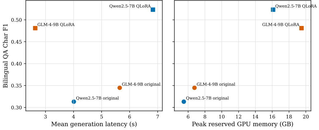
Figure 6: Bilingual QA quality against generation latency and peak GPU memory. Source: Authors’ own work.
